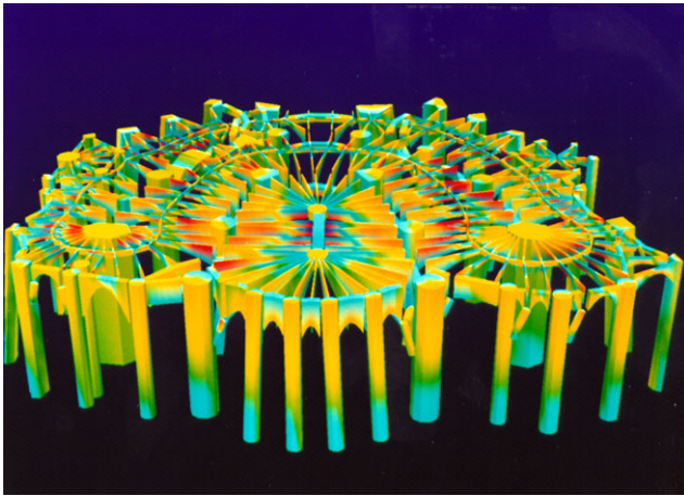
Fig. 19 (Color online) Linear elastic analysis of the Crypt of the Güell Colony near Barcelona (Roca [119]). Regions subjected to tensile normal stresses are represented in red colour
