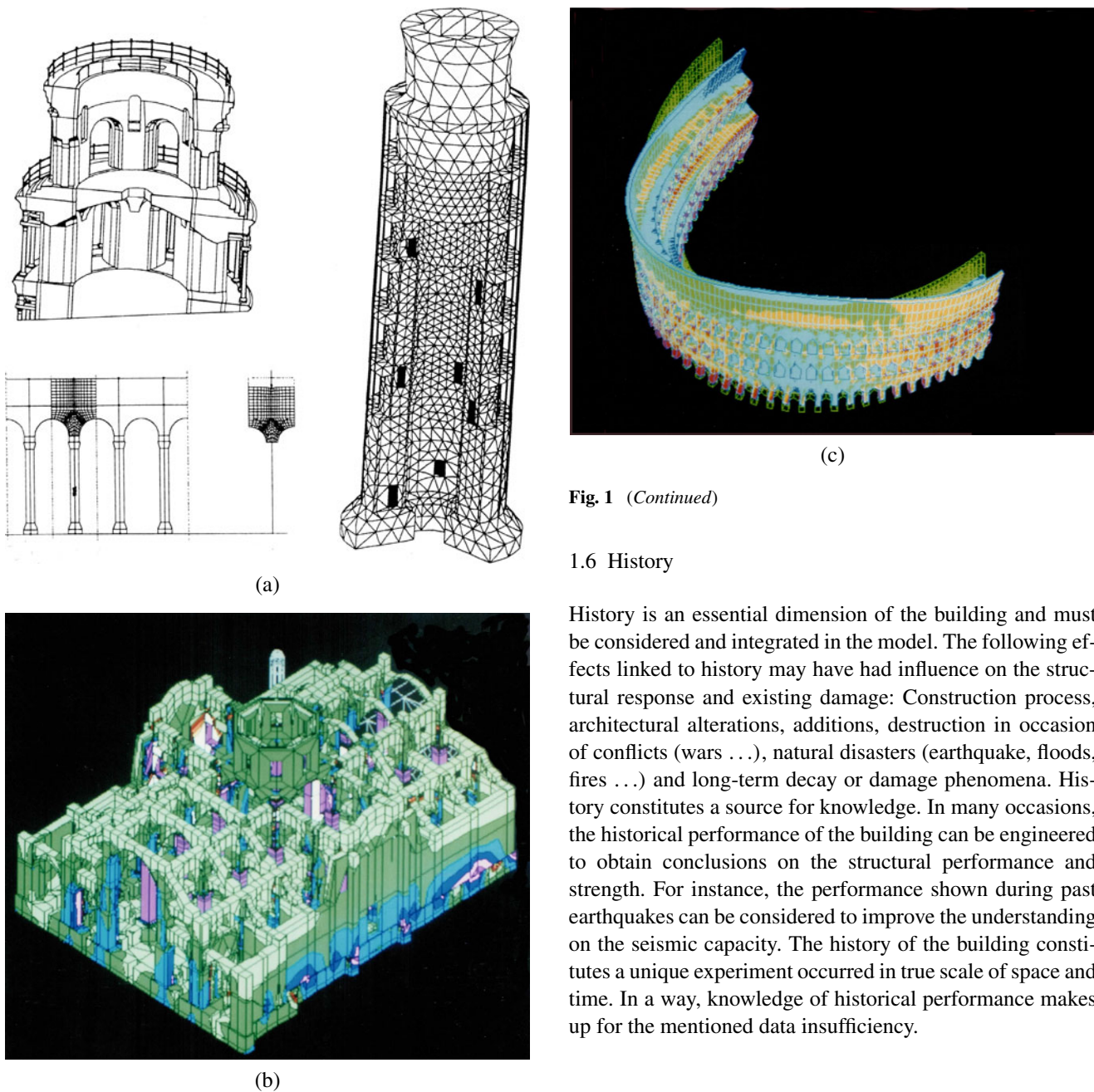
Fig. 1 Some pioneering FEM studies on historical structures. (a) Tower of Pisa: FEM model and substructuring of the colonnade system (Macchi et al. [79]). (b) Mexico City Cathedral (Meli and Sánchez Ramírez [88]). (c) The Colosseum in Rome. Tensile horizontal stresses due to the seismic action (Croci [34])
