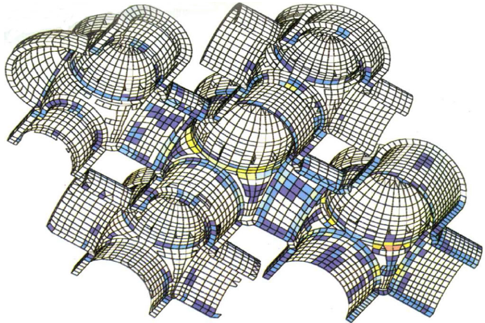
Fig. 30 Study of Saint Marco's domes in Venice by a continuum damage model (Oñate et al. [100])
