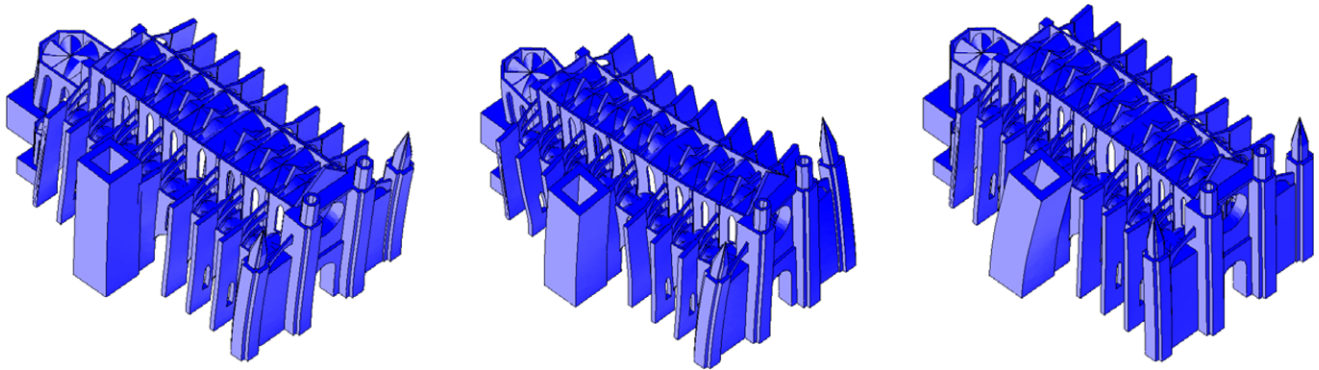
Fig. 6 Detailed modelling of Mallorca cathedral, in Spain, including the different parts of the structure which can influence on the modal analysis (tower, façade, choir) and first modal shapes (Roca et al. [126])
