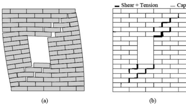
Fig. 27 Micro-modelling of masonry shear walls (Lourenço [70]). Top : Load-displacement diagram. Bottom : Results of the analysis at a lateral displacement of 2.0 mm: (a) deformed mesh; (b) damage
