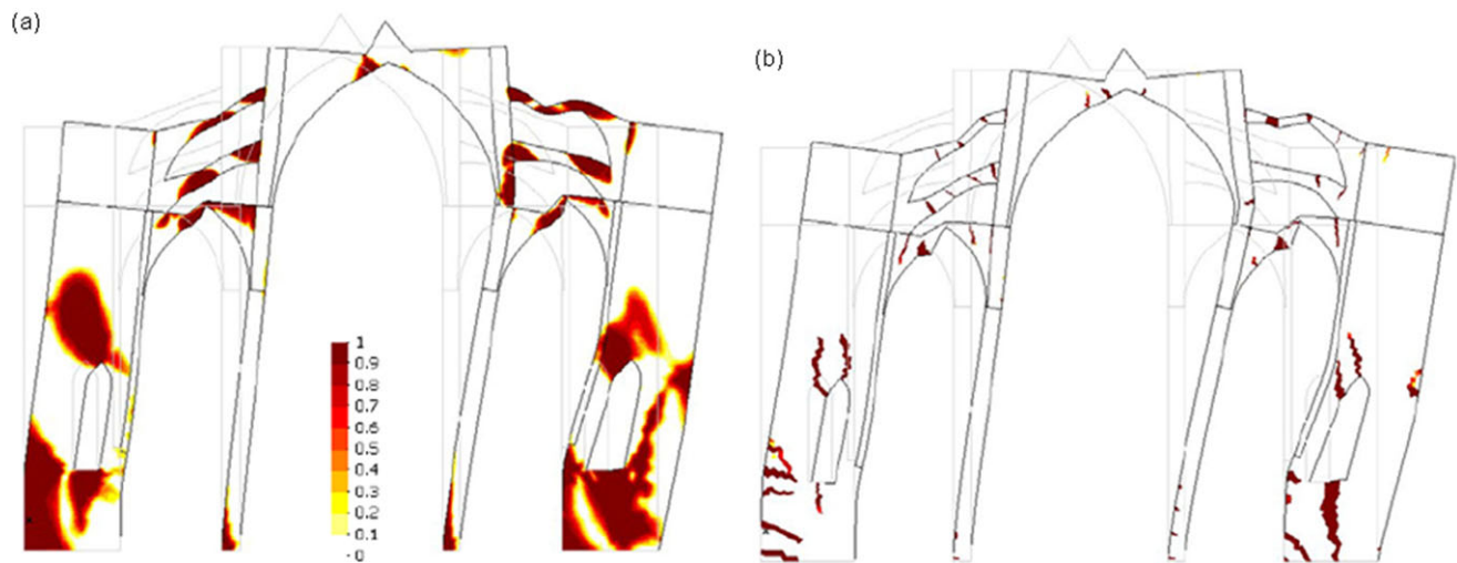
Fig. 24 Seismic analysis of Mallorca Cathedral. Smeared damage approach (a) versus localized damage approach (b), for an earthquake of 475 years of return period (Clemente et al. [31]). Both diagrams represent the tensile damage scalar parameter in chromatic scale
