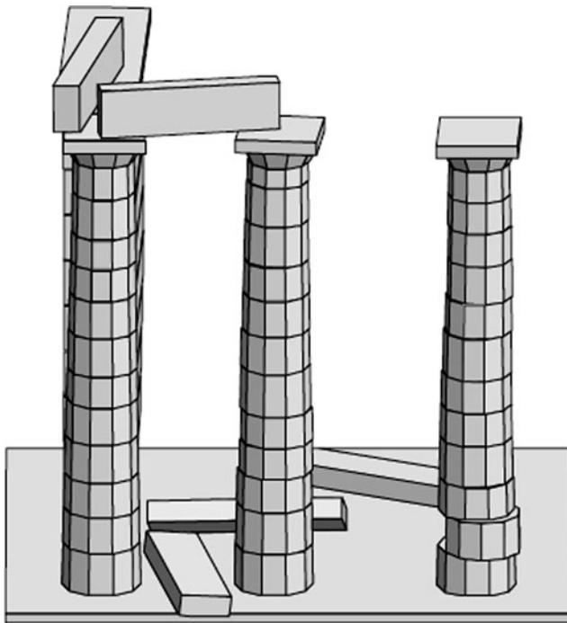
Fig. 32 Final position of the column-architrave model of the Parthenon Pronaos, without reinforcement, for a simulated earthquake (Psycharis et al. [117])
