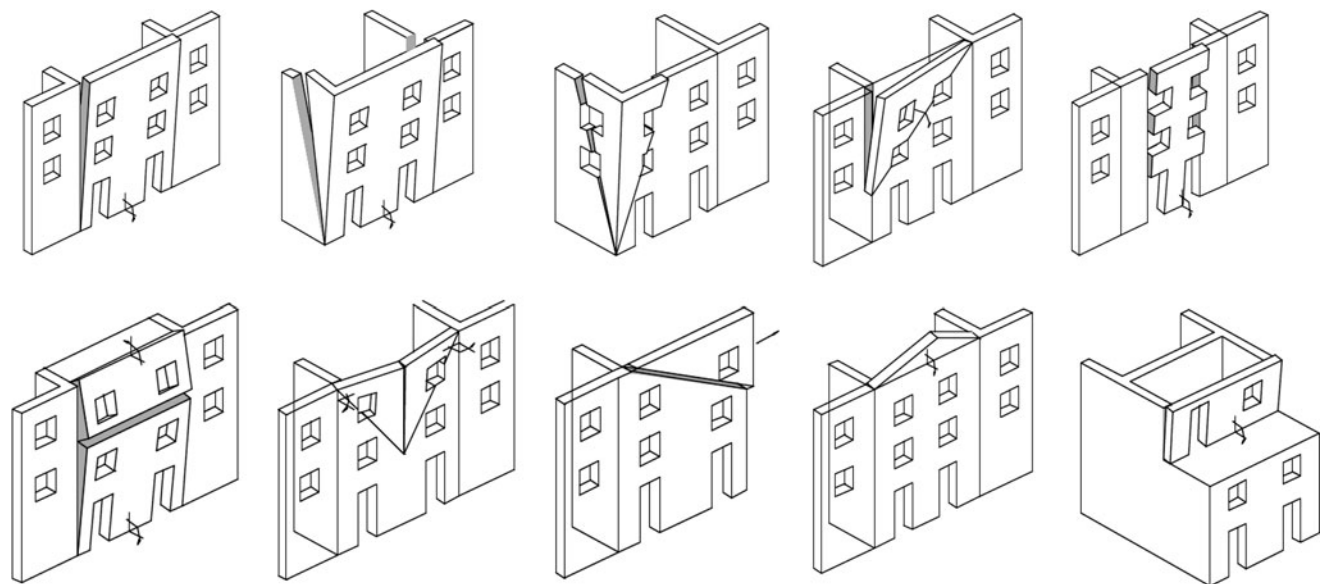
Fig. 13 Failure mechanisms for buildings embedded within urban texture (based on D'Ayala and Speranza [41])
