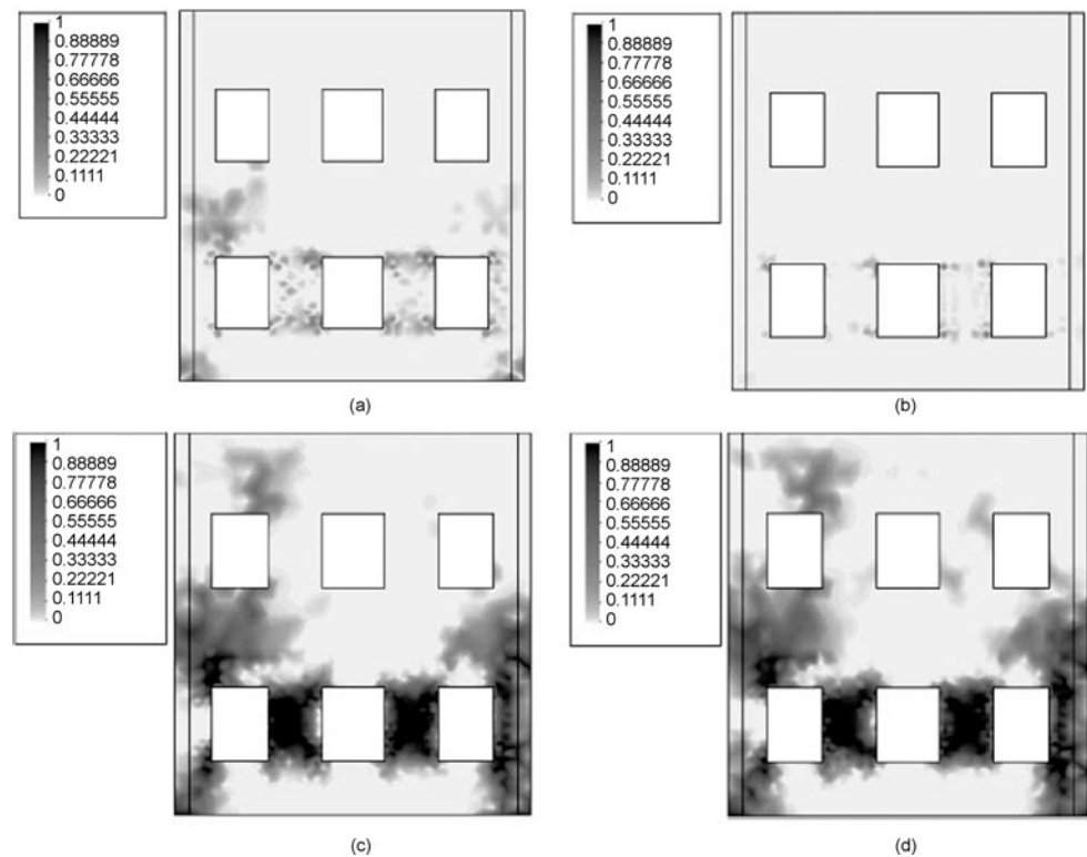
Fig. 22 Analysis of a cyclically-loaded wall with openings (from Berto et al. [9]): (a) dx- , (b) dy- , (c) dx+ and (d) dy+ numerical damage contours
