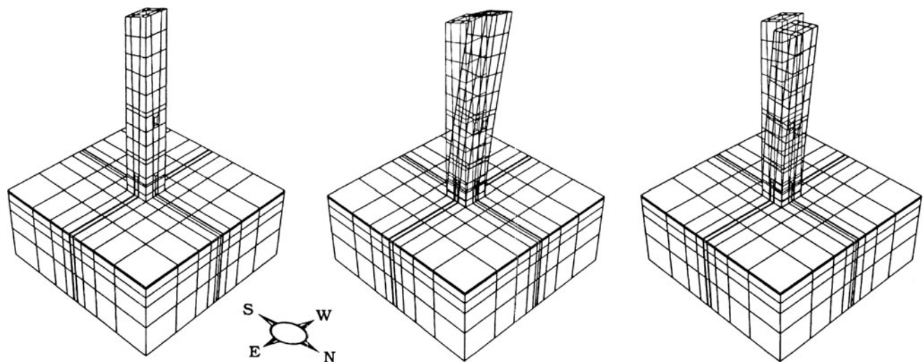
Fig. 3 Examples of graphical rendering for a FE mathematical model of a masonry tower: discretized geometry, including the soil foundation, and first two vibration modal shapes (Fanelli [44])
