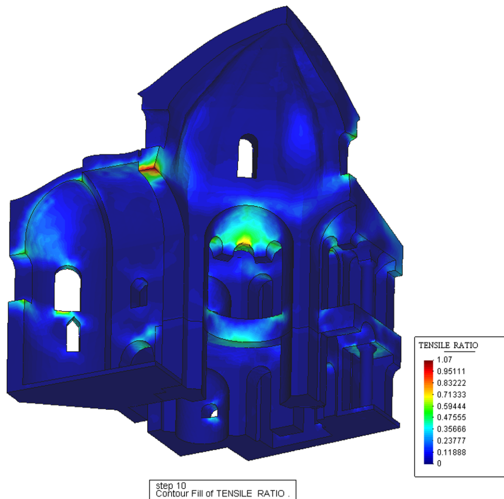
Fig. 23 (Color online) Analysis of Küçük Ayasofya Mosque in Istanbul by a damage mechanics—based macro-model. Distribution of tensile damage parameter (in chromatic scale) for the structure subjected to dead loading (Roca et al. [123])
