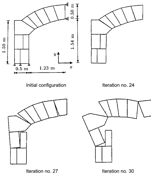
Fig. 31 Failure mode of a masonry arch (Mamaghani et al. [81])
