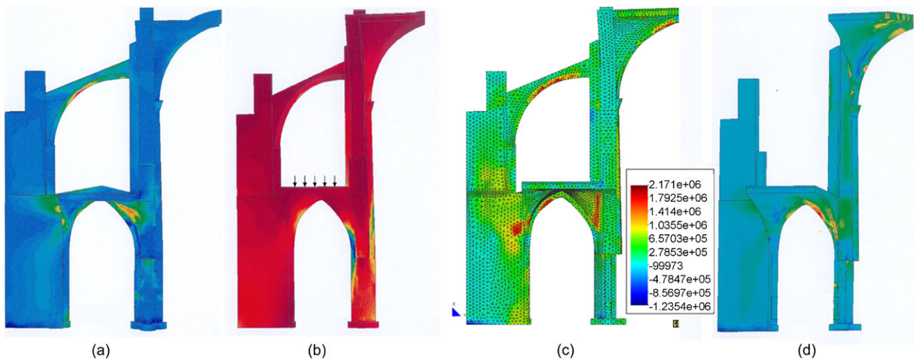
Fig. 7 (Color online) Analysis of Tarazona Cathedral for different historical configurations (Roca [121]) by FEM isotropic damage model. (a) Distribution of tensile damage at the initial condition after construction (12th–13th c.); (b) compression damage after overloading
