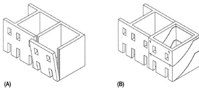
Fig. 12 Failure modes for buildings with no ties (a) and with ties anchoring the facade to lateral walls (Carocci [23])
