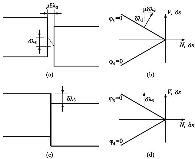
Fig. 16 Associated flow rule ( top ) with \mu = \tan \Phi = \tan \psi , and non-associated flow rule ( below ), with null dilatancy ( \tan \psi = 0 ). The yield criterion is represented as relationship between the normal ( N ) and shear forces ( V ). The corresponding displacements are the normal ( \delta n ) and tangent ( \delta s ) ones
