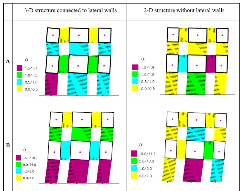
Fig. 20 Analysis with macro-blocks of a façade wall tested by Calvi and Magenes [20]. Damage distribution under monotonic loading (Brencich, Gambarotta and Lagomarsino [18]) at peak load (A) and at the end of the monotonic load history (B)
