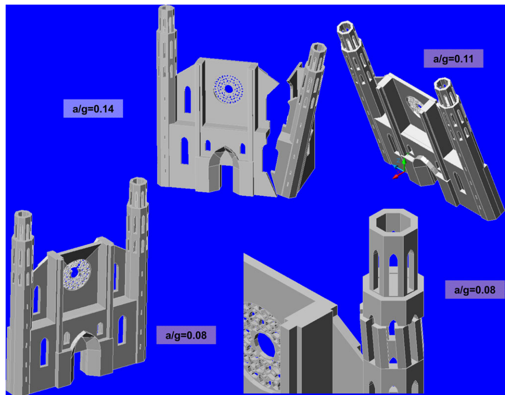
Fig. 14 Kinematic analysis applied to possible collapse models of the façade of Santa Maria del Mar church in Barcelona (Roca et al. [126])
