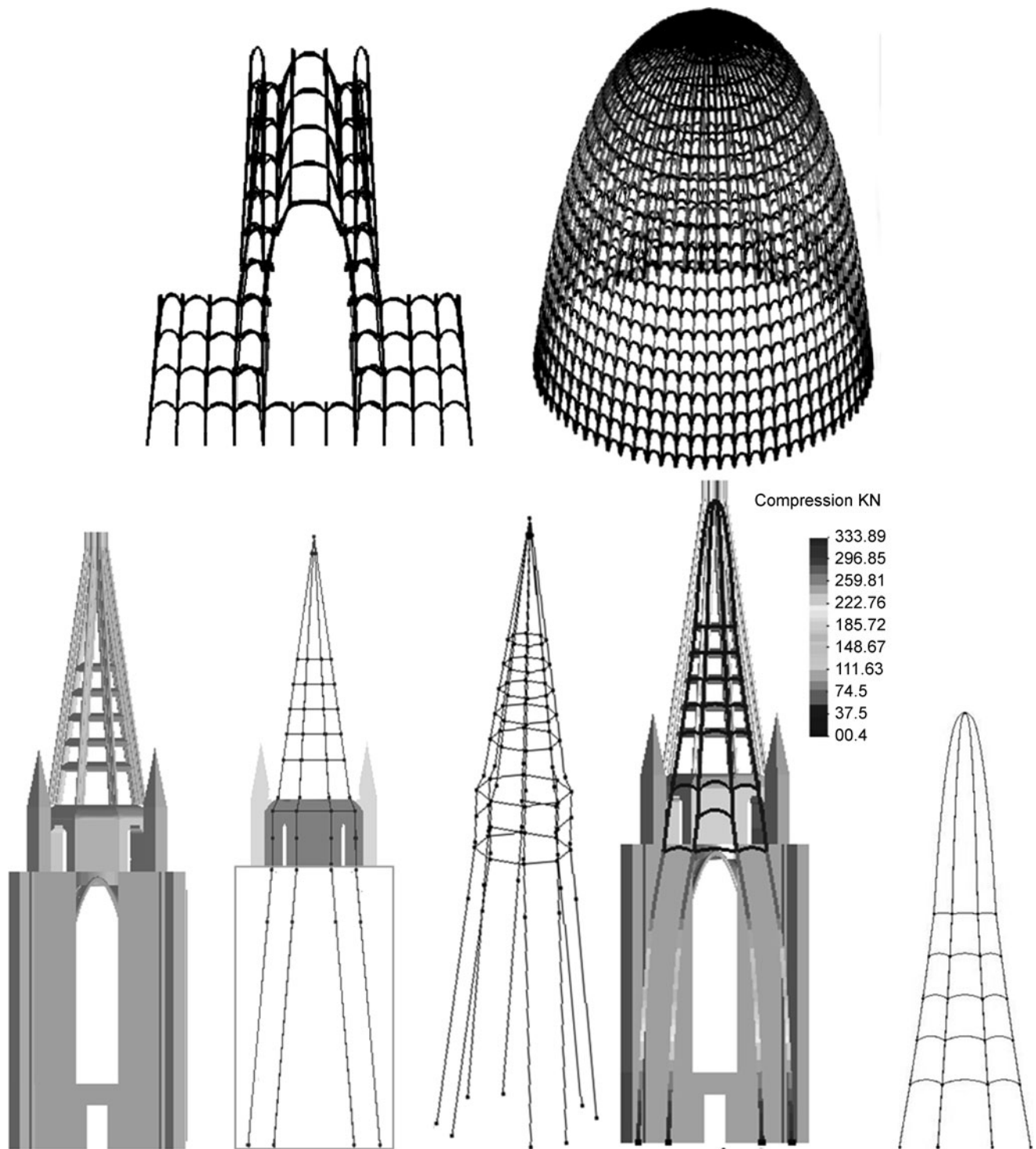
Fig. 18 Examples of inverted multiple nets ( top ) and application to describe the equilibrium condition of a tower of the façade of Barcelona Cathedral (Andreu et al. [2])
