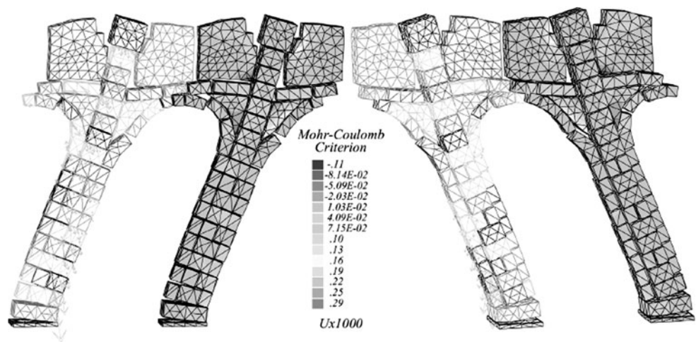
Fig. 25 3D failure mechanism of part of the cloister of São Vicente de Fora Monastery in Lisbon as obtained by Pegon et al. [111]
