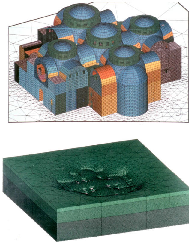
Fig. 2 The finite element model of the St. Mark's Basilica: Top : global discretization; Bottom : soil foundation discretization including deformation (Mola and Vitaliani [93])
