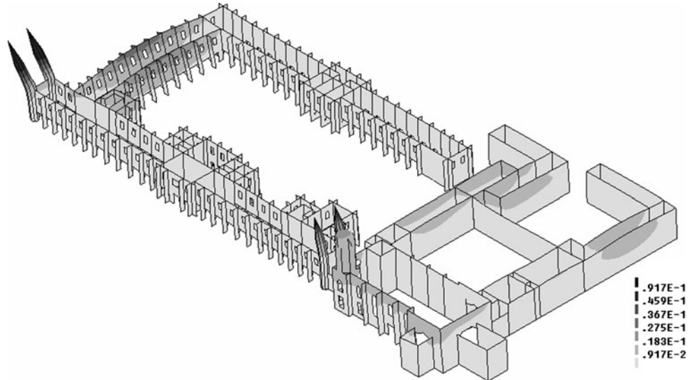
Fig. 5 Deformed meshes and maximum displacements (in grey scale) for seismic load acting along the longitudinal direction of the building. Monastery of Jerónimos (Lourenço and Mourão [72])
