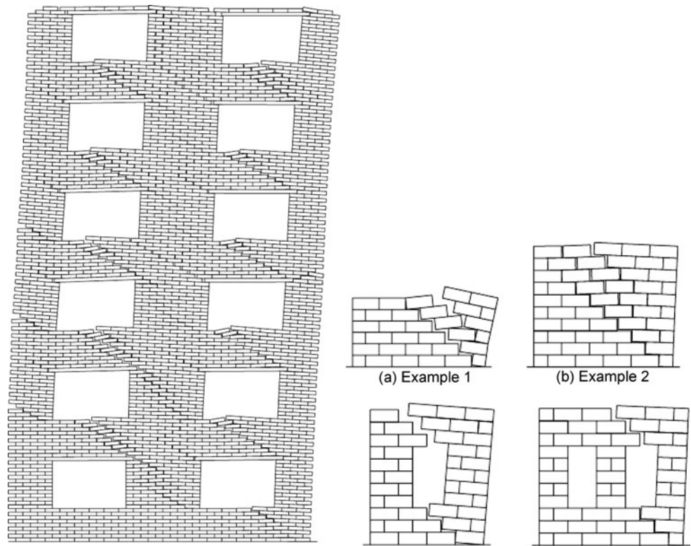
Fig. 17 Failure modes for walls subjected to vertical and horizontal loading obtained by Gilbert et al. [50]
