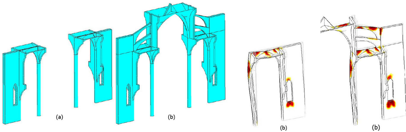
Fig. 8 Sequential analysis of Mallorca Cathedral taking into account the construction process (Clemente [31]) using a FEM isotropic damage model. Phases considered ( left ) and corresponding distribution of deformation and damage ( right )
