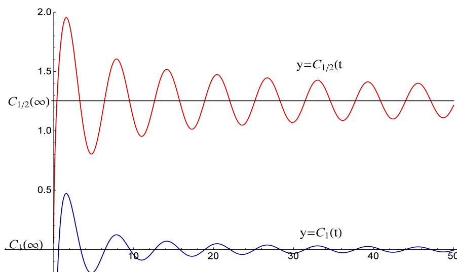
Figure 2: Graphs of C_1(t) , C_{1/2}(t) .
